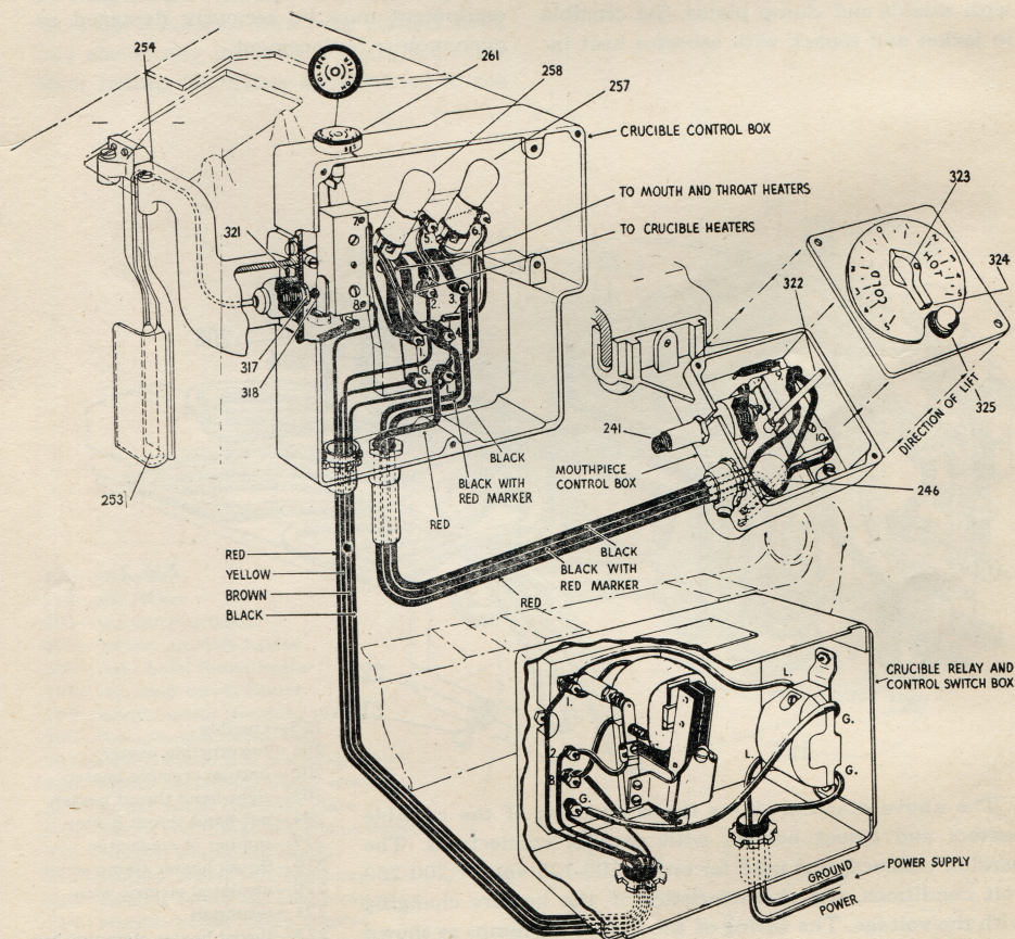
Wiring Diagram for 110 Volts A.C.
