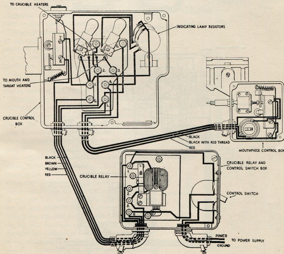
Wiring Diagram for 220 Volts A.C.
