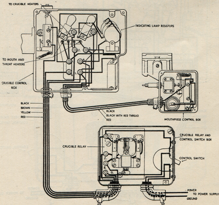
Wiring Diagram for 220 Volts D.C.
