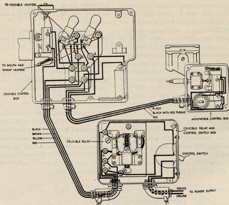
Wiring Diagram for 110 Volts D.C.
