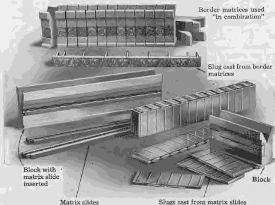
FIG. 59-1. Border matrices, matrix slides, and slugs cast from them.
