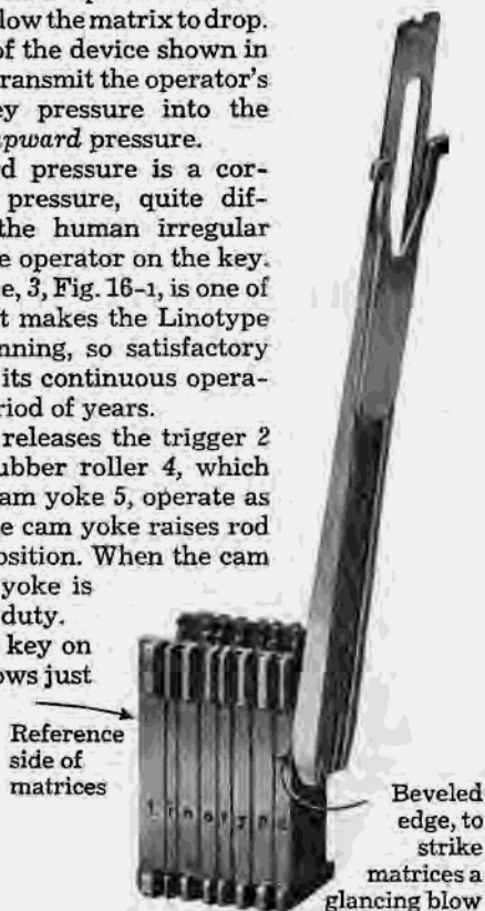
FIG. 8-1. View of spaceband dropping into line of matrices.
