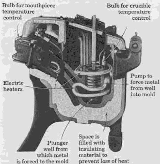
FIG. 41-1. Cross section of Linotype electric pot.
