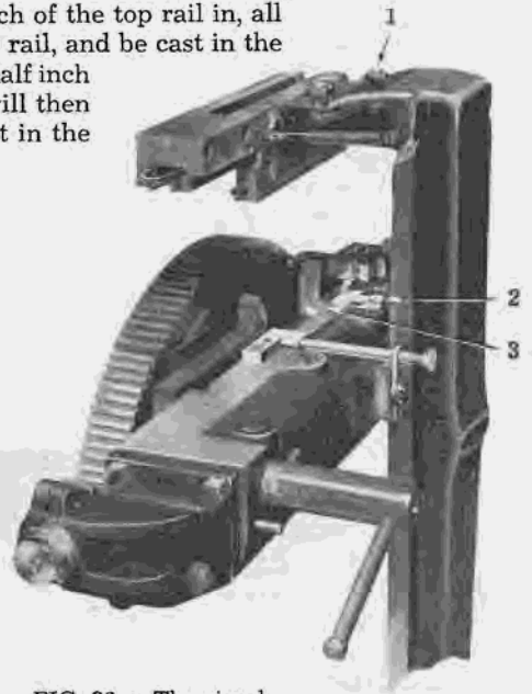
FIG. 36-1. The simple two-letter attachment. Adjusting screw 1 comes down on point 2, when this attachment is in use, and prevents the first elevator from descending farther. The matrices are thus held higher than usual, and the cast is made from their auxiliary characters.
