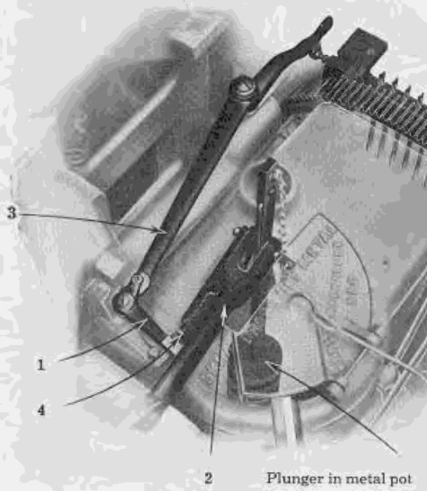
FIG. 43-1. The pot pump stop. Arm 1, which locks the pump lever 2, does not move back and allow pump lever to descend unless the front part of operating lever 3 is pressed to the right by a completely filled line of matrices and spacebands. If arm 1 has not moved back, catch block 4 on pump lever comes in contact with arm 1 and keeps the pump lever from descending.
