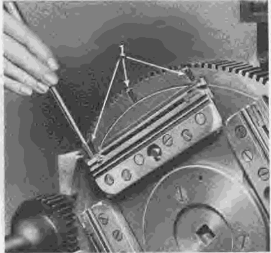
FIG. 34-1. View of method of changing mold liners.
