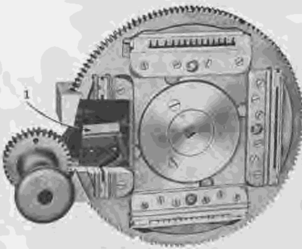
FIG. 45-1. View of mold disk with section removed to show back knife.
