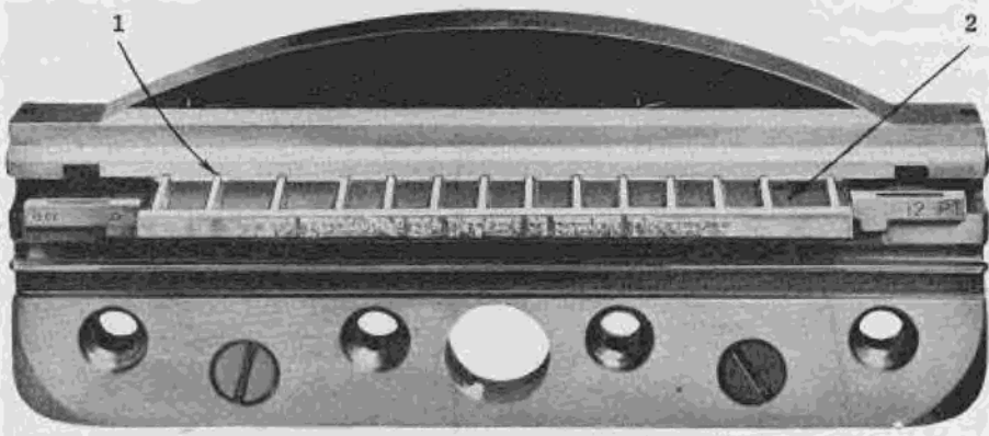
FIG. 31-1. Recessed mold.
