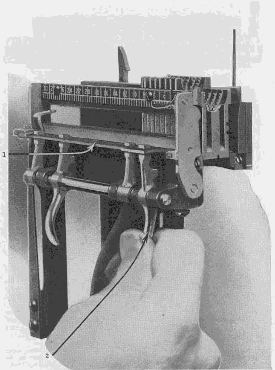
FIG. 26-1. This view indicates aligning and casting level. Assembled in this manner top characters of the lower matrices and bottom characters of the raised matrices will be cast in the same line.
