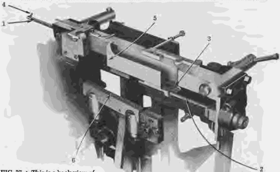
FIG. 37-1. This is a back view of the vise-like jaws between which the matrices and spacebands are held while they are in the casting position in front of the mold. The mold disk, of course, is not shown here as it would make this view impossible.
