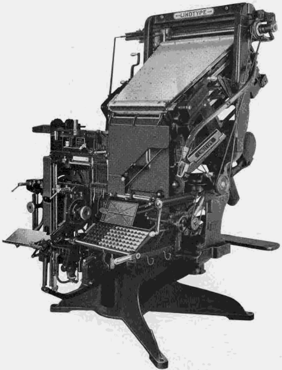
FIG. 1-1. A Model 31 four-magazine Linotype. Many of the detail illustrations in this book are based upon this model. There are variations for specific purposes in other models, but the big scheme of simple operation applies to every Linotype.
