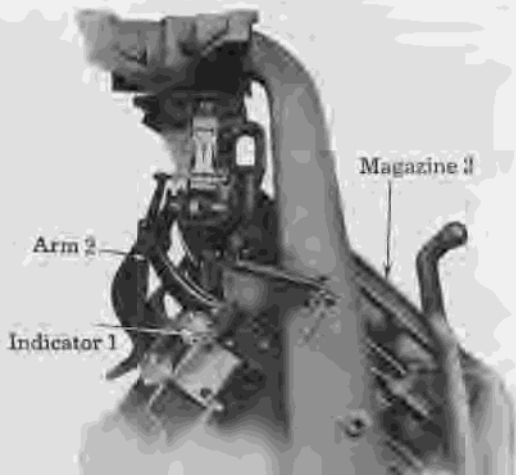
FIG. 55-1. View of font distinguisher shows how the position of the arm 2 determines the front-to-back position of the vertical knife-like projection in the bottom of the distributor box.
