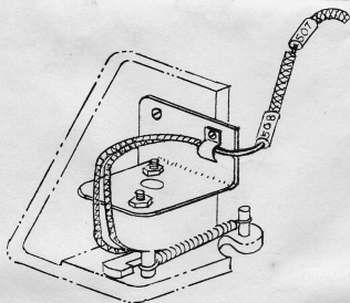
E-5908 POT PUMP SOLENOID BRACKET, ASSEM.
