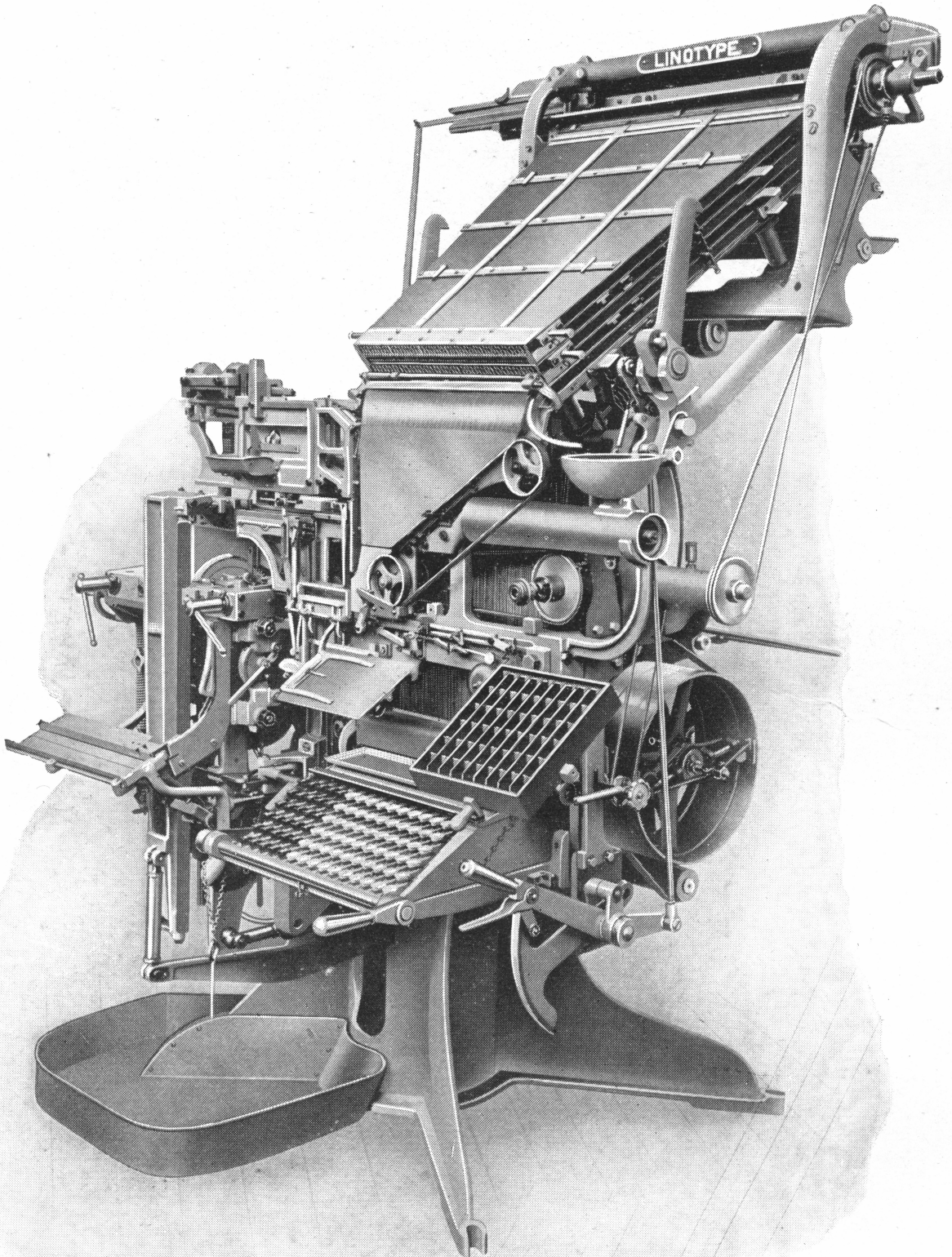
FIG. 408.— Linotype; treble magazine machine; English model 4; front view.
