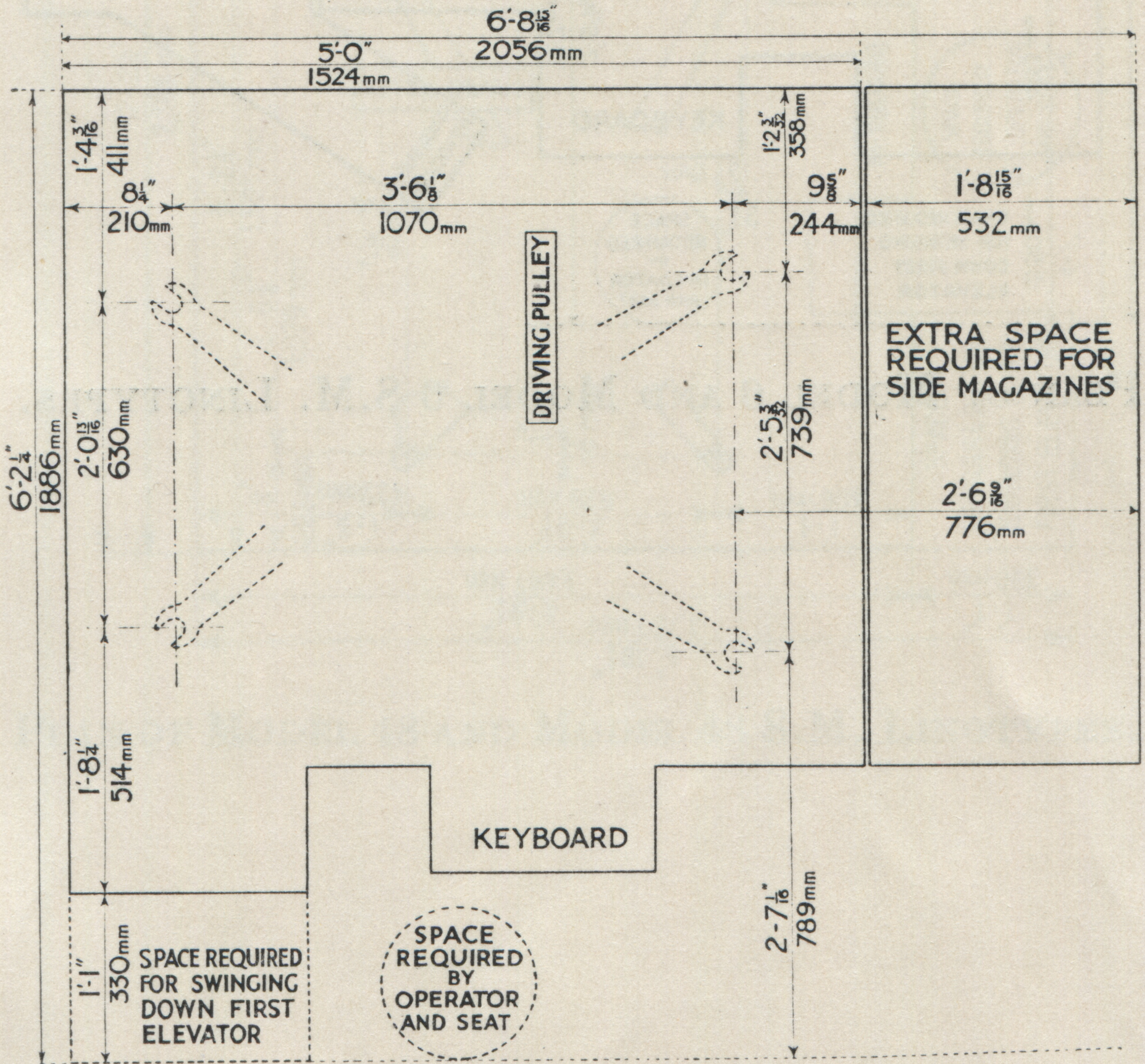
PLAN OF MODEL 4 AND MODEL 4 S.M. LINOTYPES.
