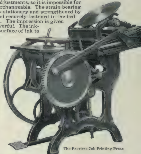
The Peerless Job Printing Press
