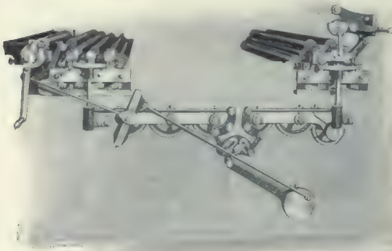
The Unequal Distribution; note the independent vibratory mechanism
