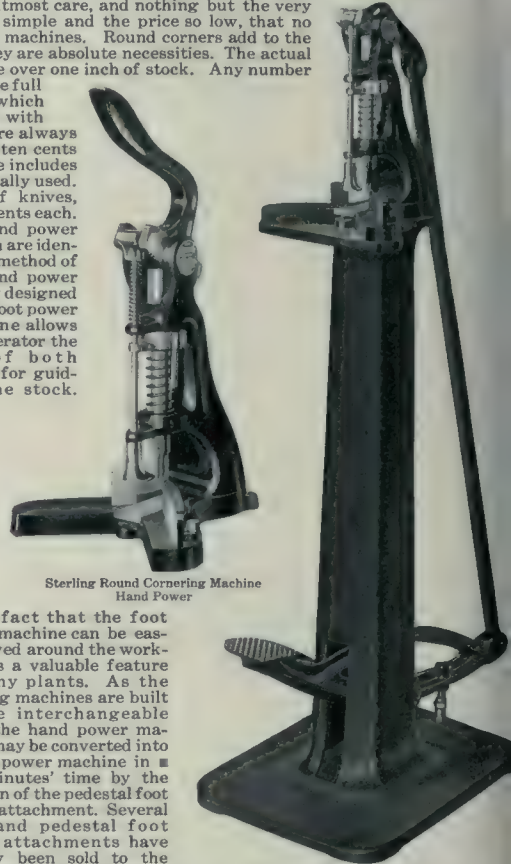
Sterling Round Cornering Machine Foot Power
