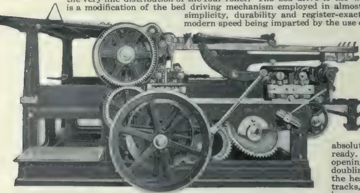
The Whitlock Two-Revolution Three-Roller Pony Press
