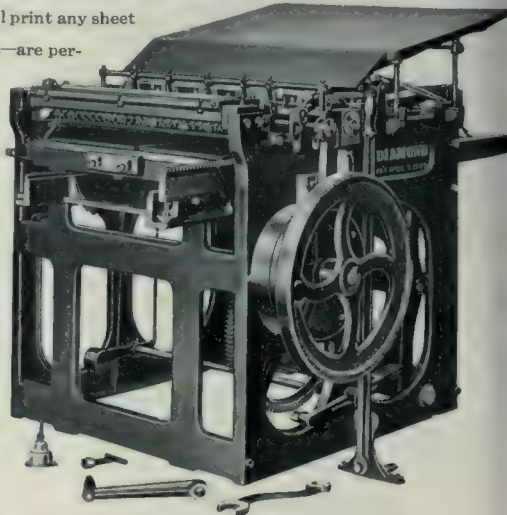
Diamond Cylinder Press
