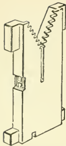
A Linotype Matrix
