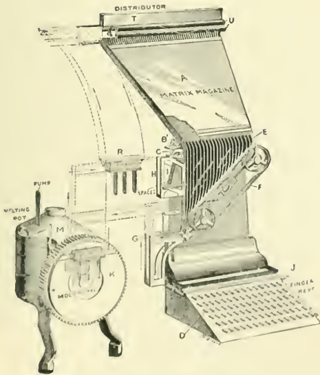
Diagram of the Linotype Machine
