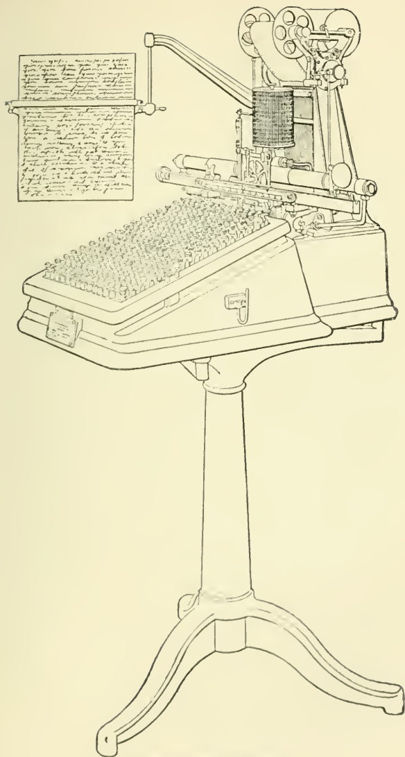
The Monotype Keyboard
