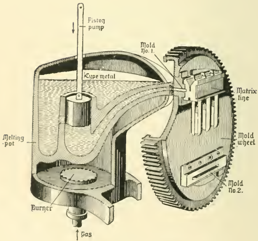
The Linotype Melting Pot and Mold Wheel
